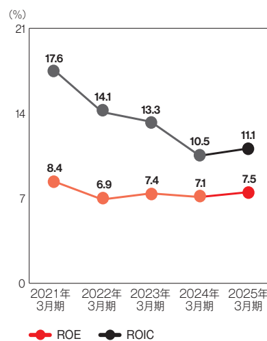
ROE、ROIC
